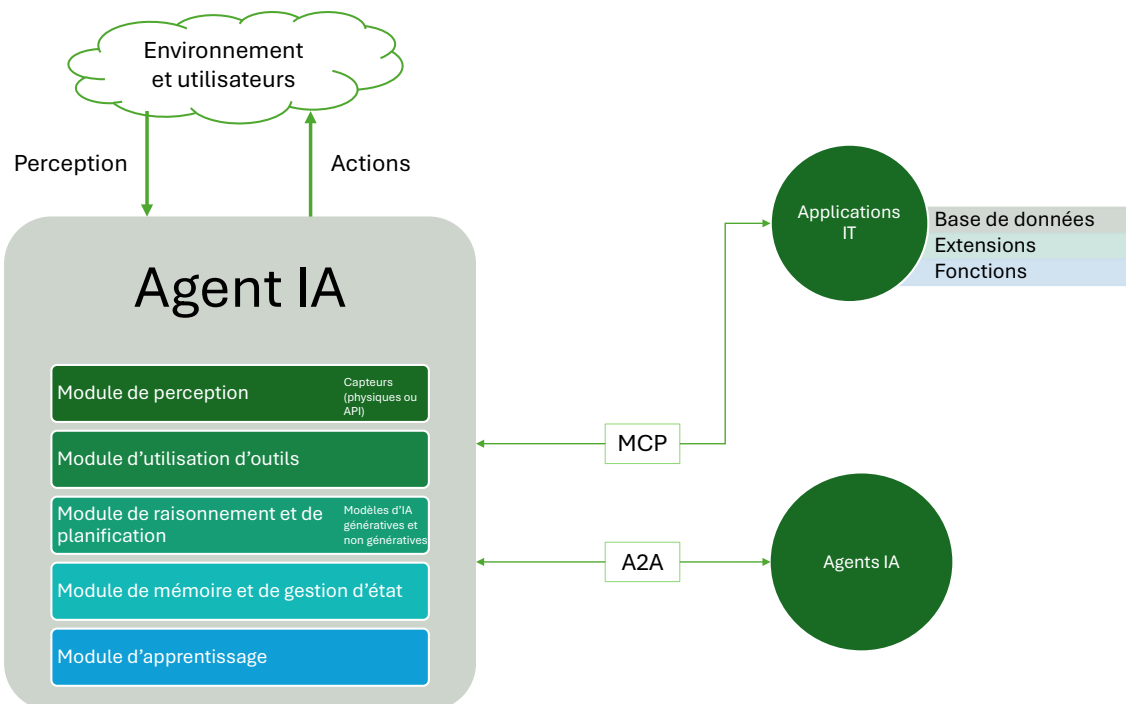
Figure 2: Architecture d'un agent IA
