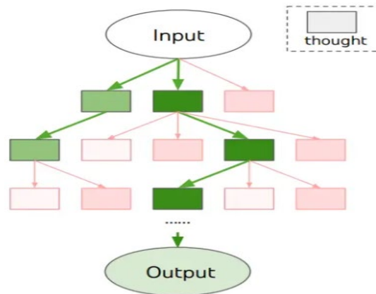
Figure 5: Schéma Tree-of-Thoughts (ToT) 83 .
